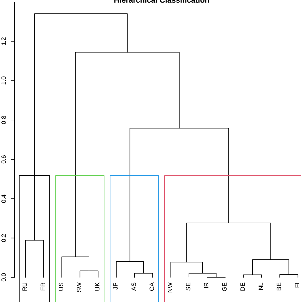
Hierarchical Classification
